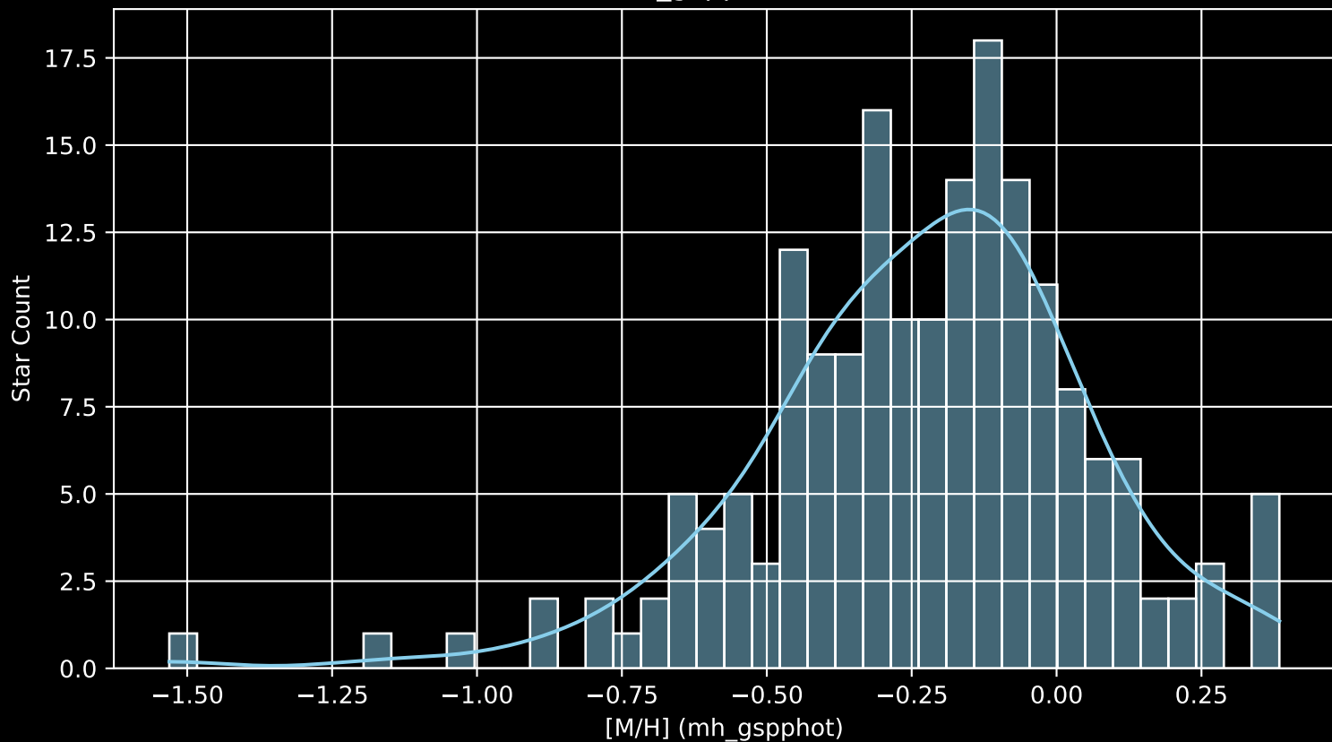
APOGEE DR17 Field: [CVZTILE_102+35_btx [M/H] (mh_gspphot) (n= 182)
