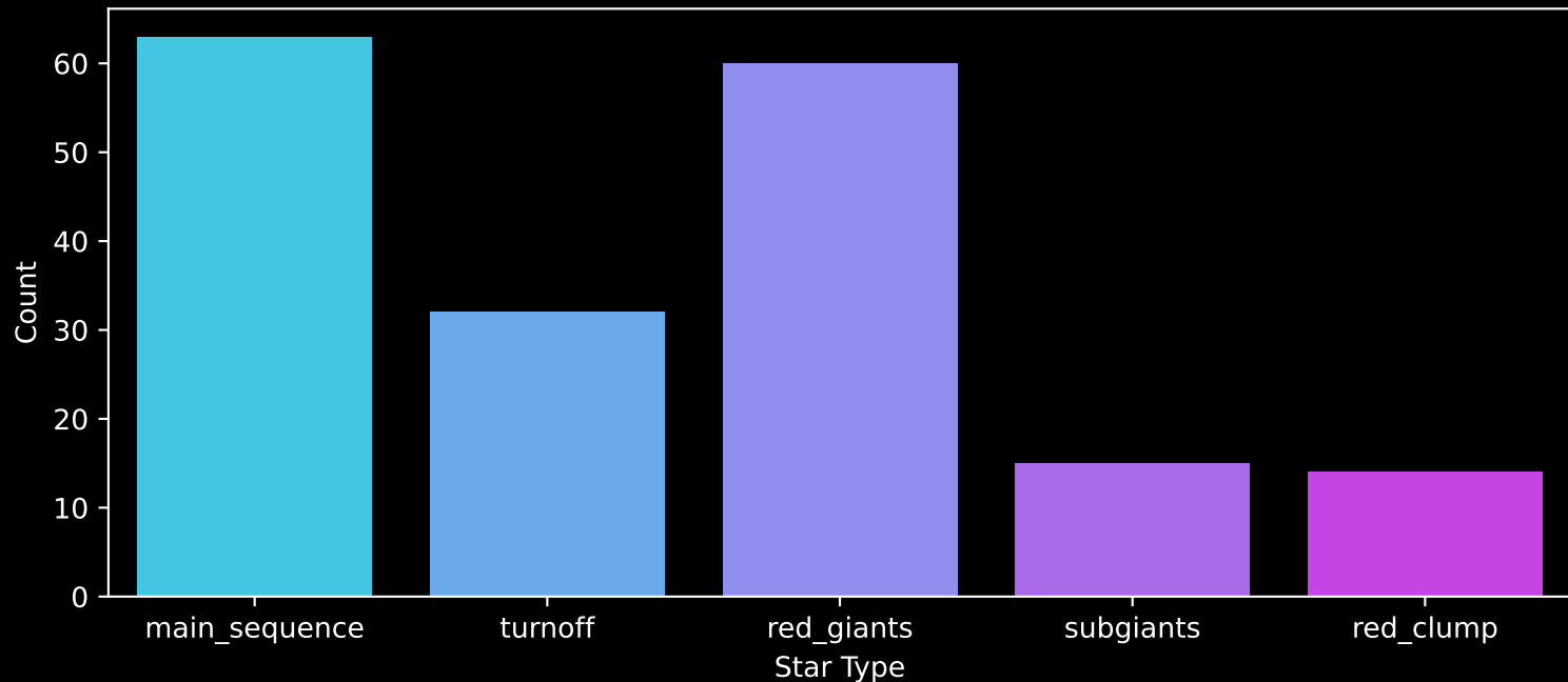
APOGEE DR17 Field: [CVZTILE_102+35_btx] Count plot of Star Type
