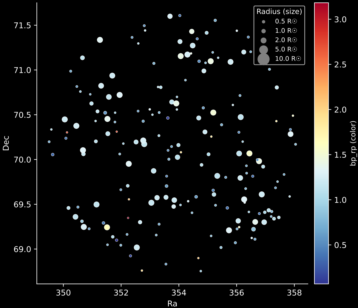
APOGEE DR17 Field: [CVZTILE_102+35_btx] Stars: 184
