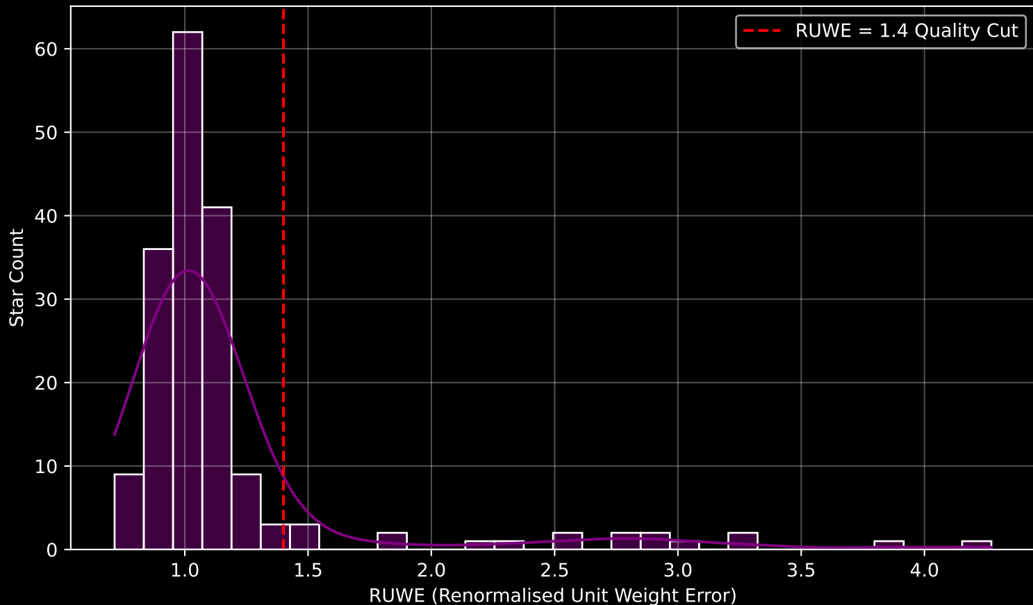
GAPOGEE DR17 Field [CVZTILE_102+35_btx] RUWE Distribution (n= 178)
