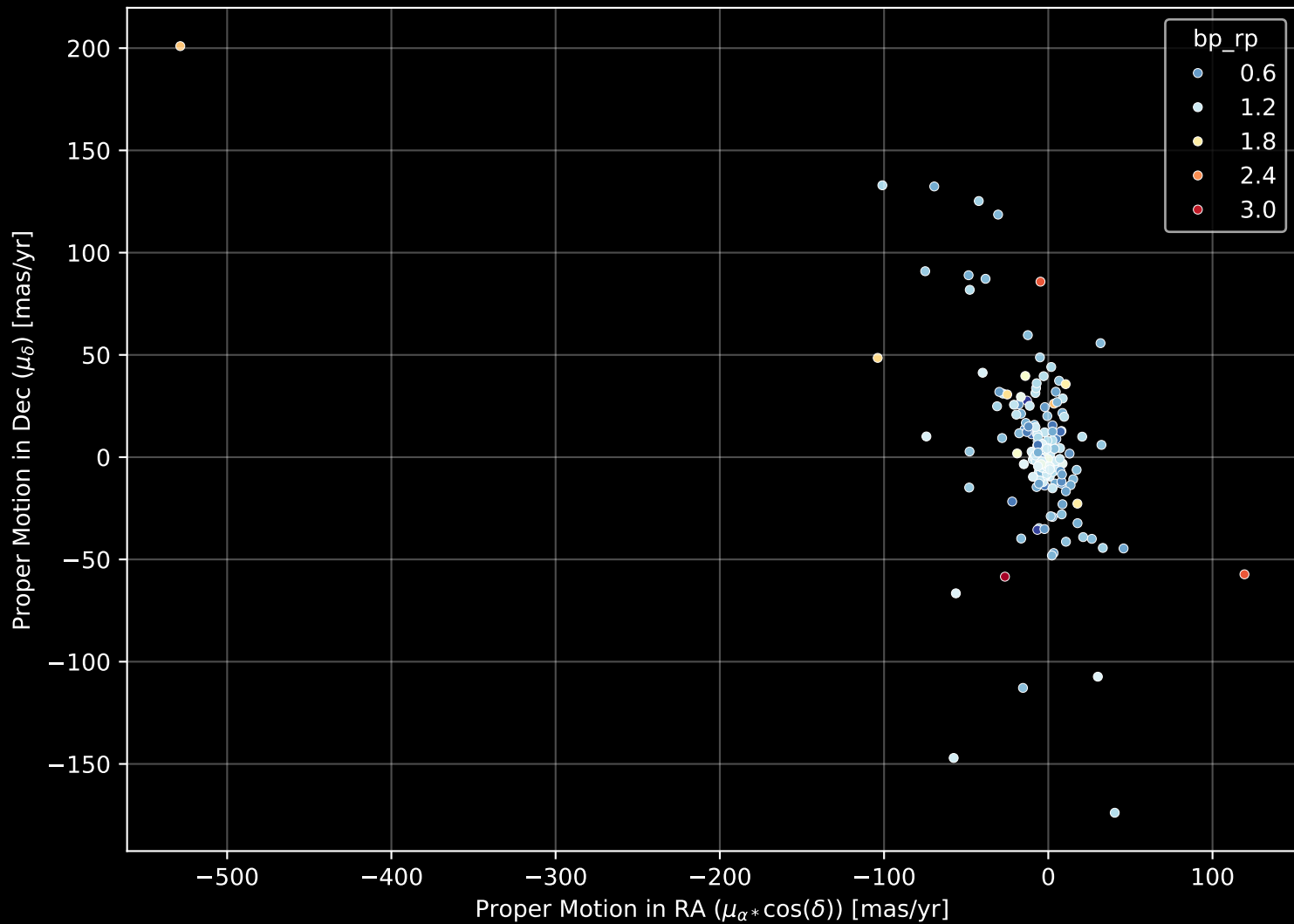
APOGEE DR17 Field: [CVZTILE_102+35_btx] Proper Motion Diagram (n= 184)
