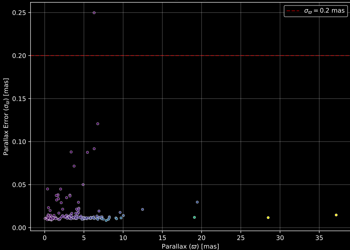
APOGEE DR17 Field: [CVZTILE_102+35_btx] Parallax Quality (n= 184)
