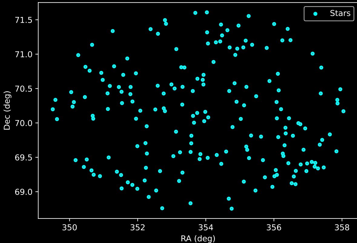
APOGEE DR17 Field: [CVZTILE_102+35_btx] Proper Motion Vectors for Gaia Star Field (n= 184)
